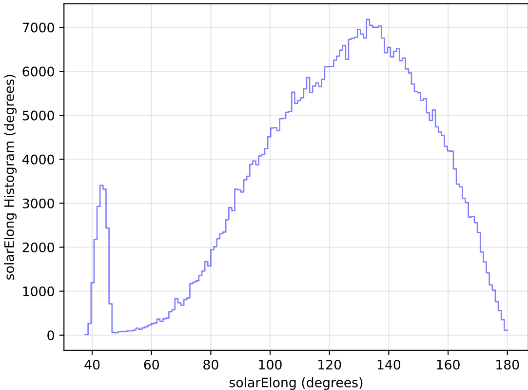
too_100_1v3.4_10yrs All sky r band: solarElong Histogram
