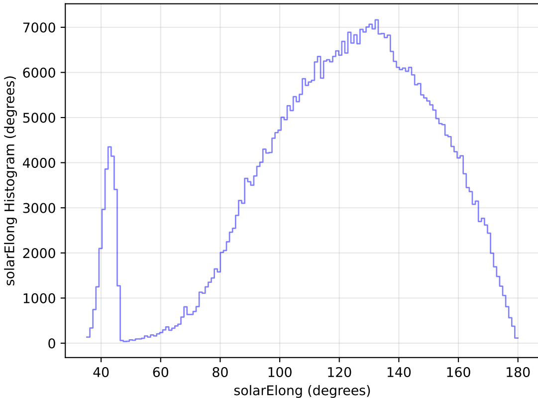
too_100_1v3.4_10yrs All sky i band: solarElong Histogram
