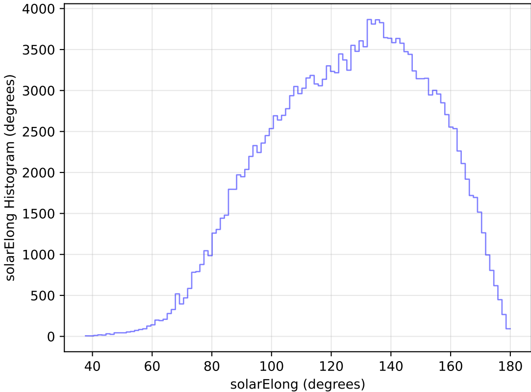
too_100_1v3.4_10yrs All sky g band: solarElong Histogram
