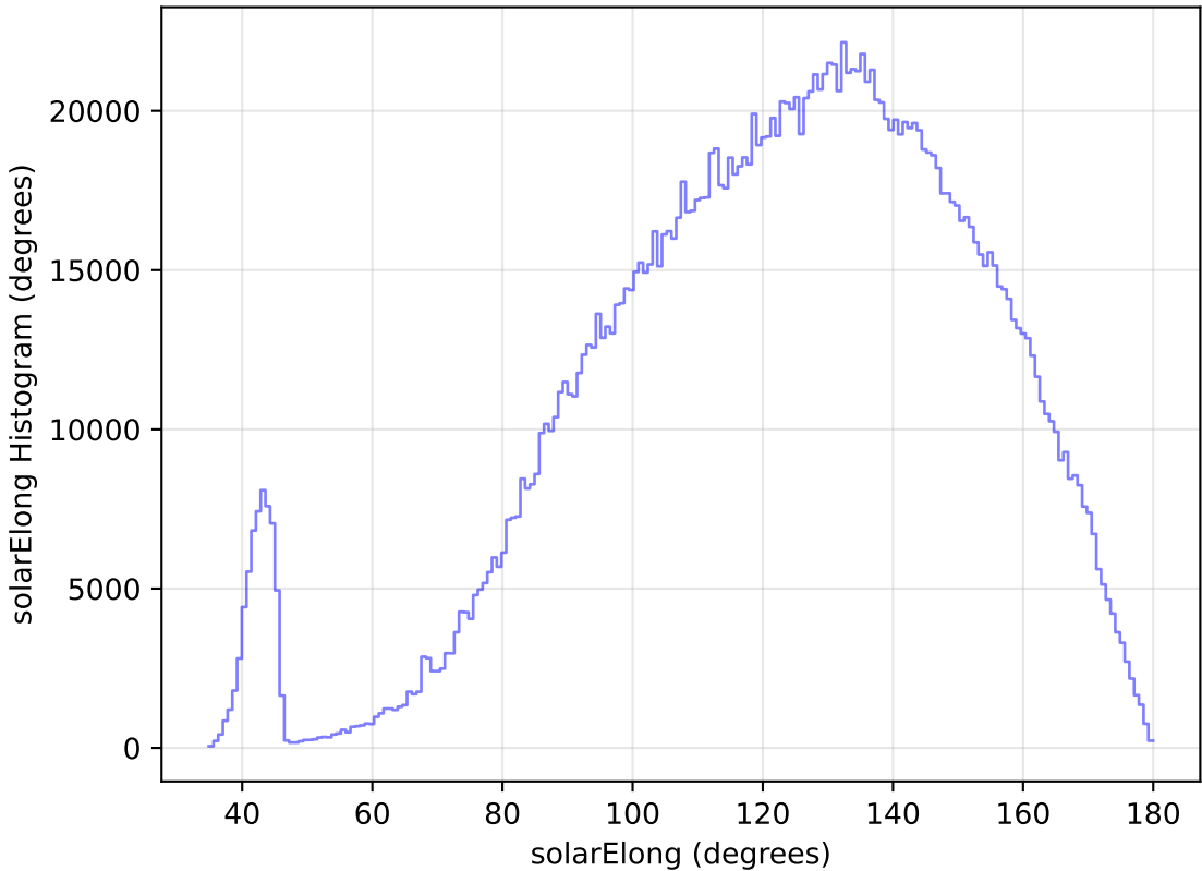
too_100_1v3.4_10yrs All sky all bands: solarElong Histogram
