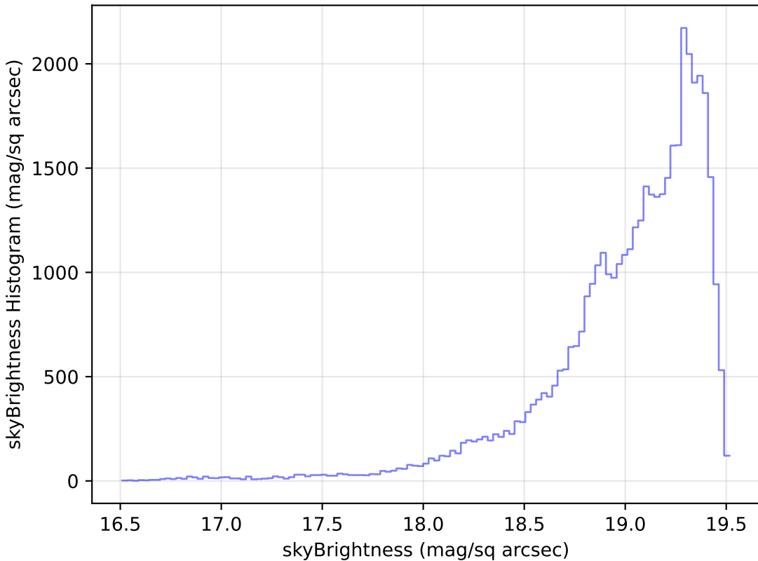
too_100_1v3.4_10yrs Yr 1 z band: skyBrightness Histogram
