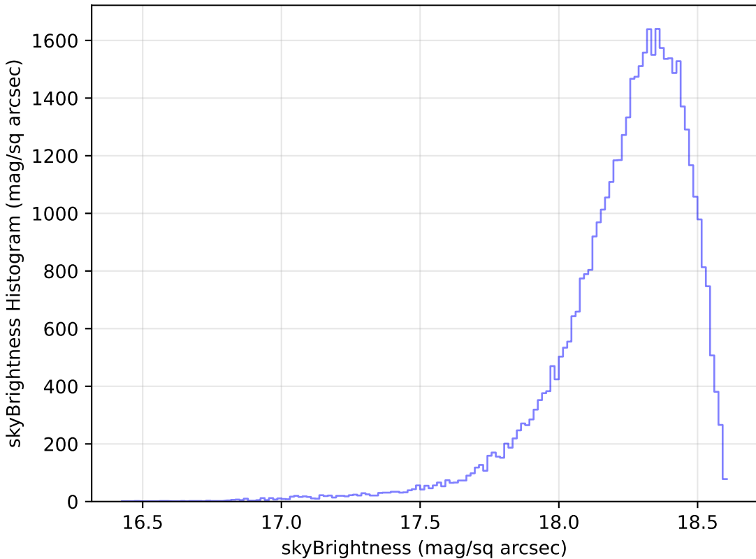
too_100_1v3.4_10yrs Yr 1 y band: skyBrightness Histogram
