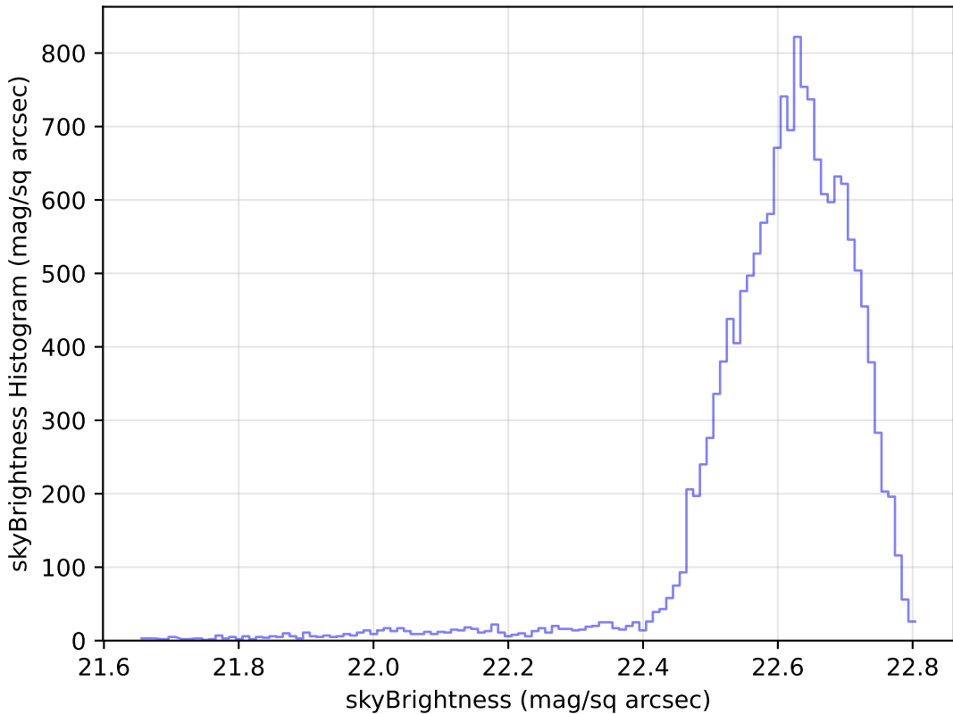
too_100_1v3.4_10yrs Yr 1 u band: skyBrightness Histogram
