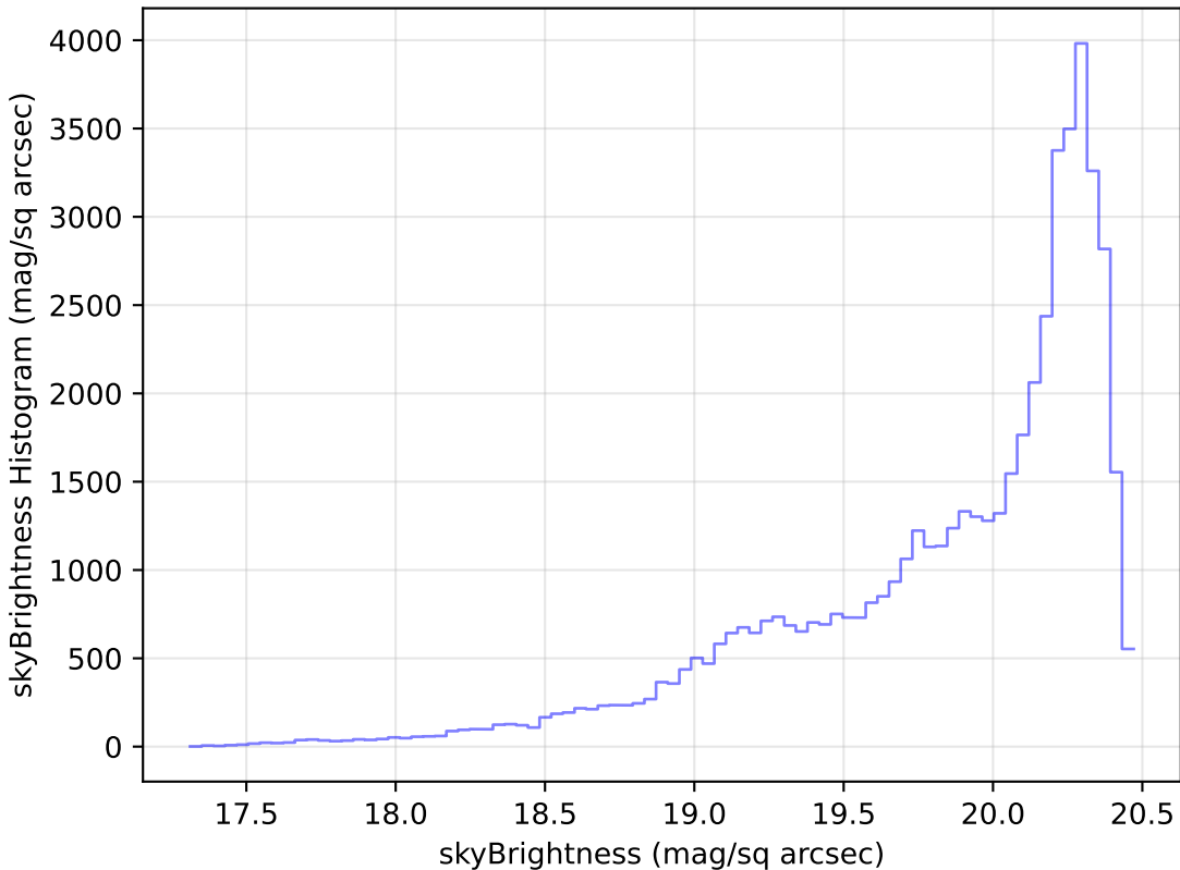
too_100_1v3.4_10yrs Yr 1 i band: skyBrightness Histogram
