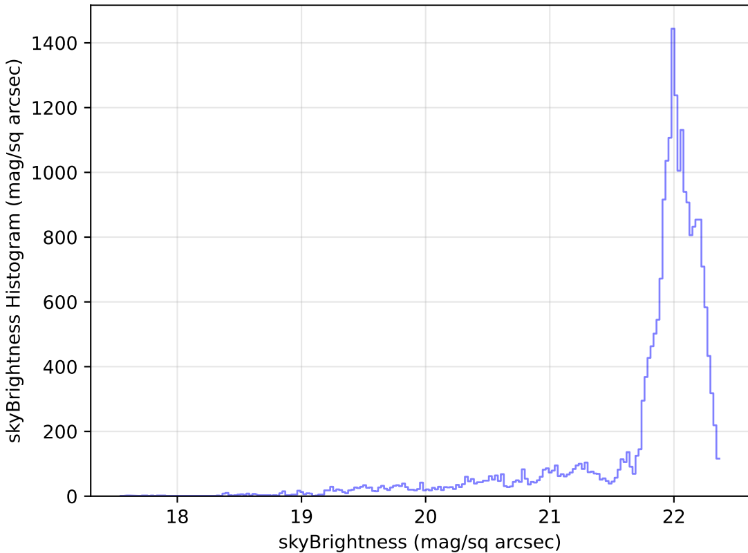
too_100_1v3.4_10yrs Yr 1 g band: skyBrightness Histogram
