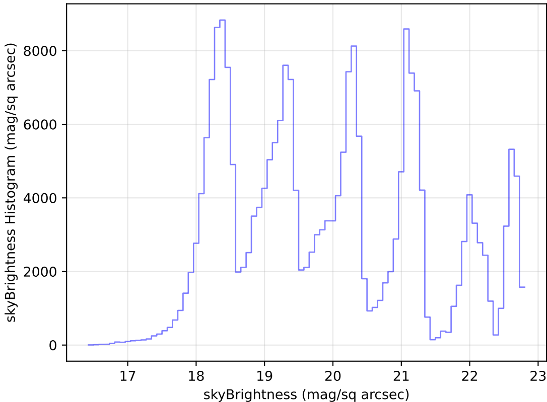
too_100_1v3.4_10yrs Yr 1 all bands: skyBrightness Histogram
