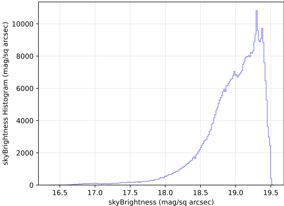
too_100_1v3.4_10yrs WFD z band: skyBrightness Histogram
