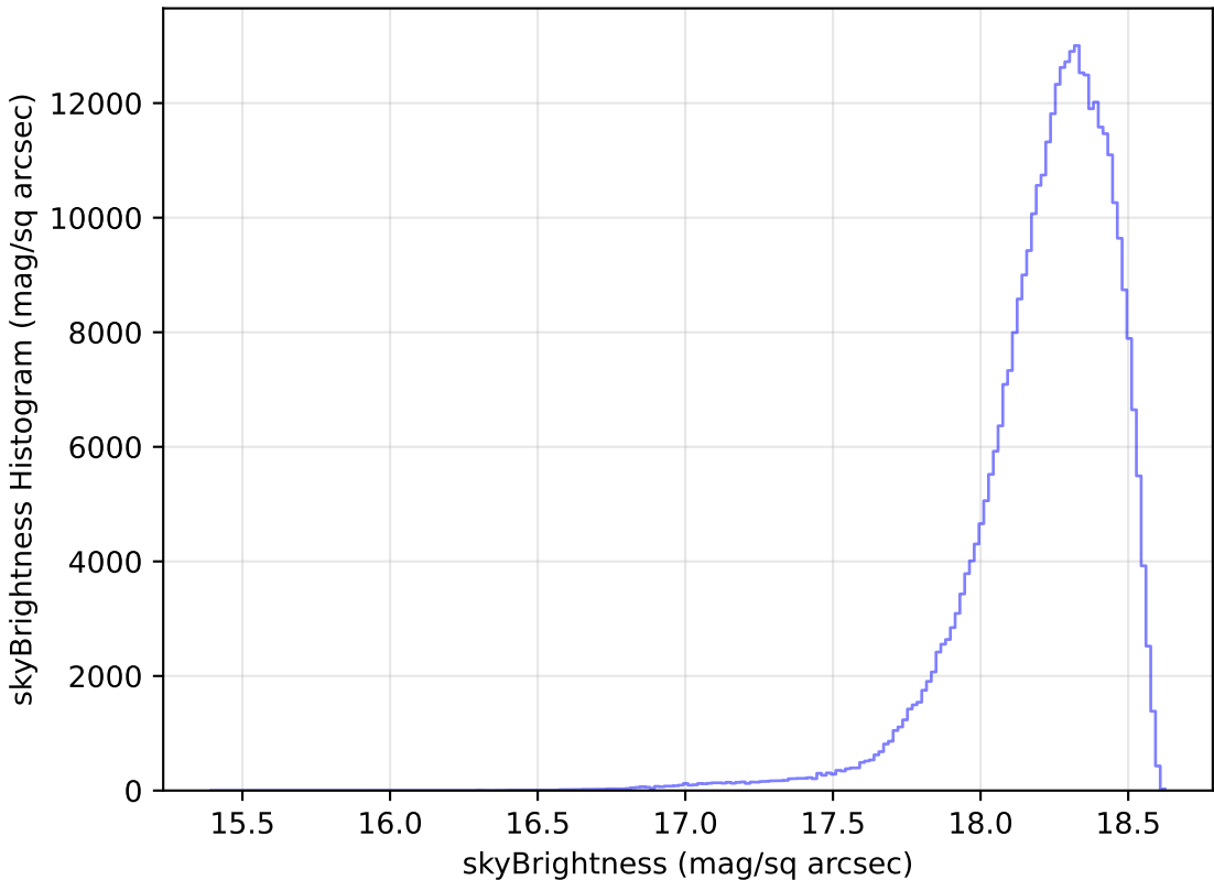
too_100_1v3.4_10yrs WFD y band: skyBrightness Histogram
