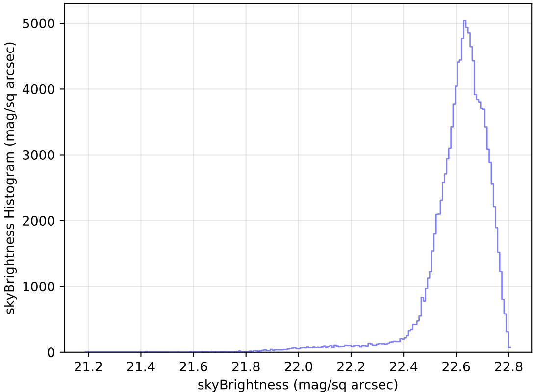
too_100_1v3.4_10yrs WFD u band: skyBrightness Histogram
