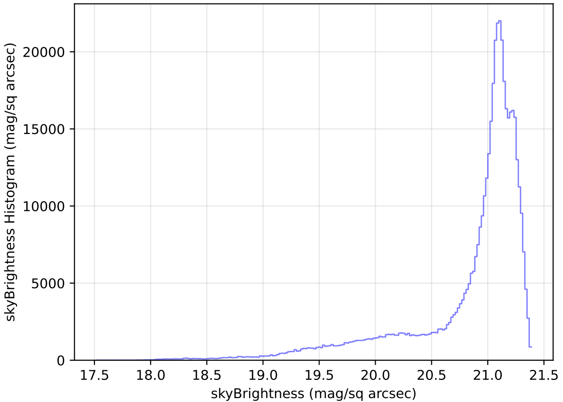
too_100_1v3.4_10yrs WFD r band: skyBrightness Histogram
