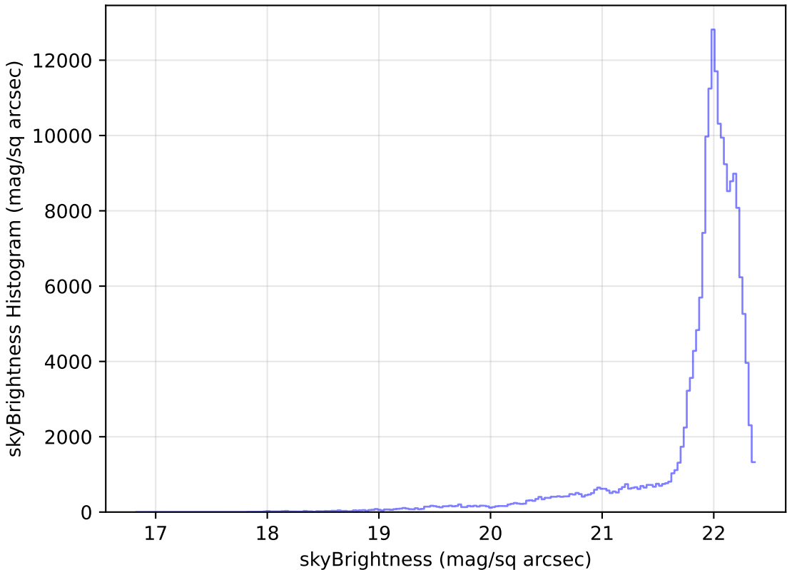
too_100_1v3.4_10yrs WFD g band: skyBrightness Histogram
