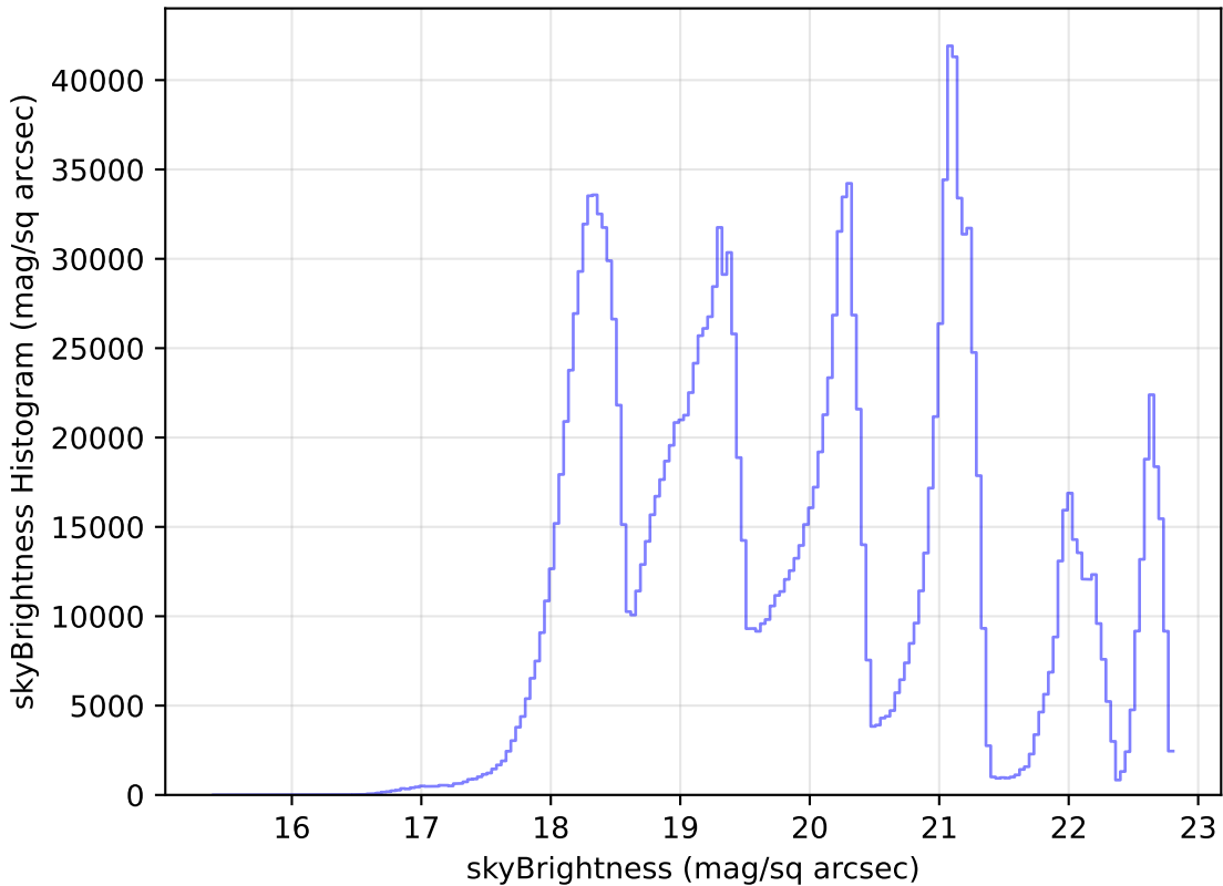
too_100_1v3.4_10yrs WFD all bands: skyBrightness Histogram
