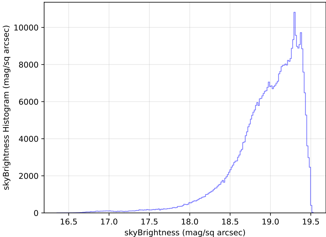
too_100_1v3.4_10yrs All sky z band: skyBrightness Histogram
