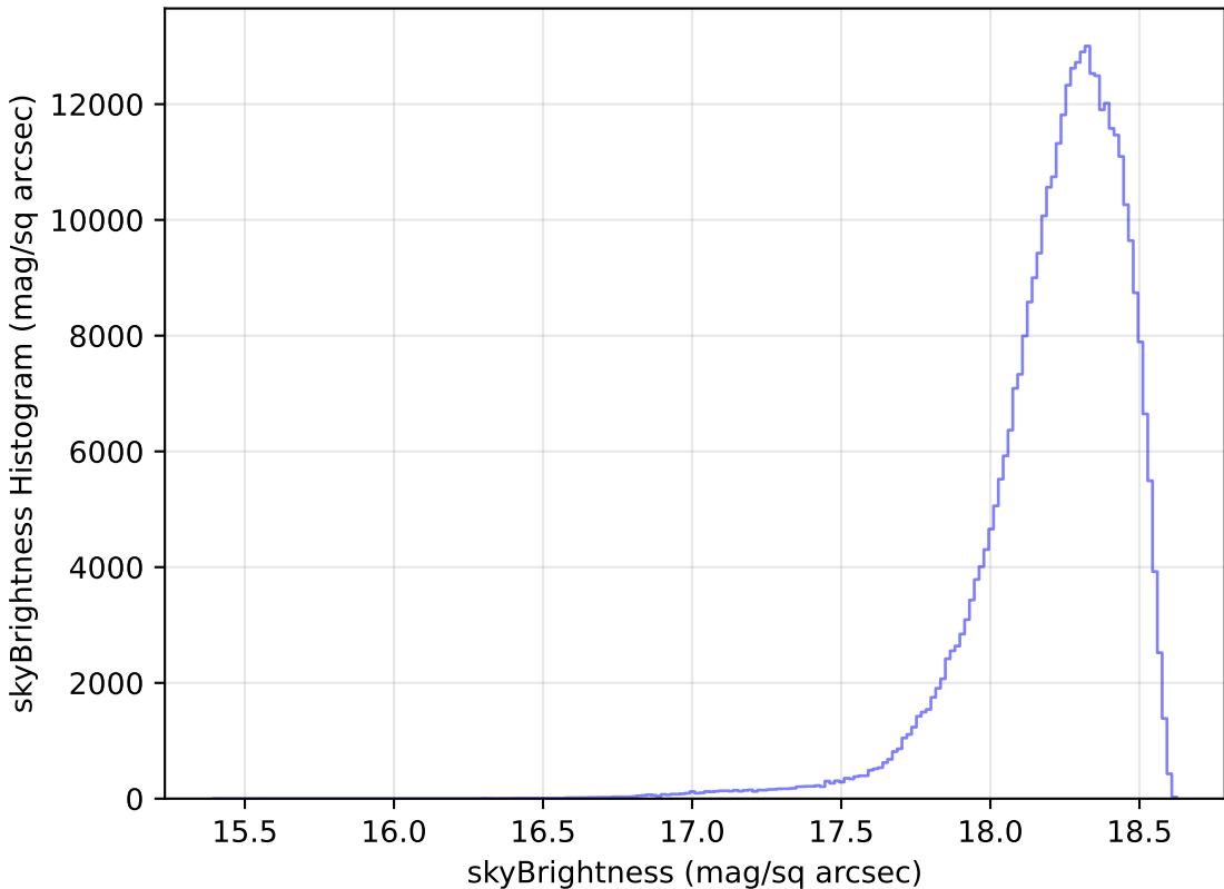
too_100_1v3.4_10yrs All sky y band: skyBrightness Histogram
