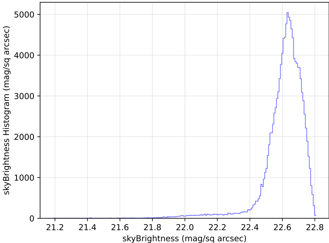
too_100_1v3.4_10yrs All sky u band: skyBrightness Histogram
