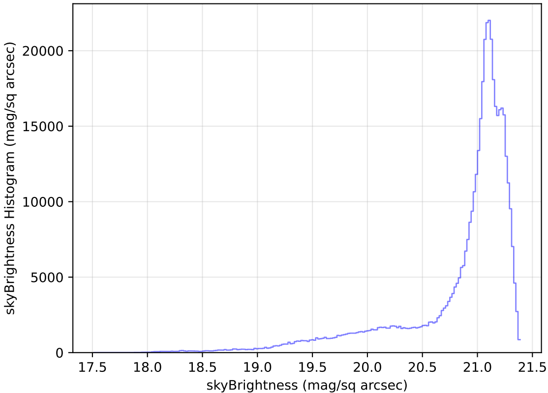
too_100_1v3.4_10yrs All sky r band: skyBrightness Histogram
