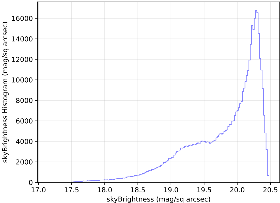
too_100_1v3.4_10yrs All sky i band: skyBrightness Histogram
