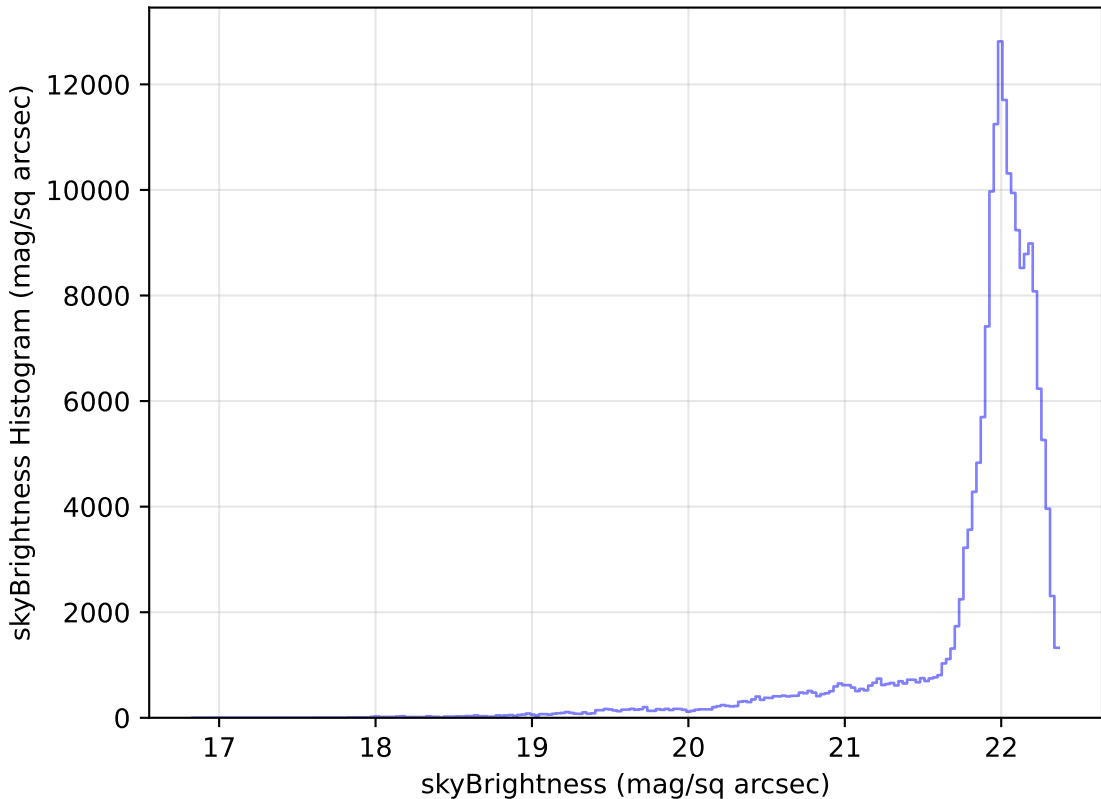
too_100_1v3.4_10yrs All sky g band: skyBrightness Histogram
