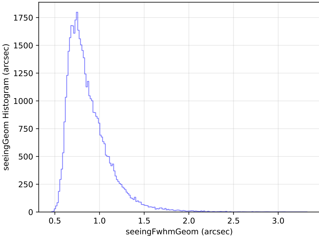
too_100_1v3.4_10yrs Yr 1 z band: seeingGeom Histogram
