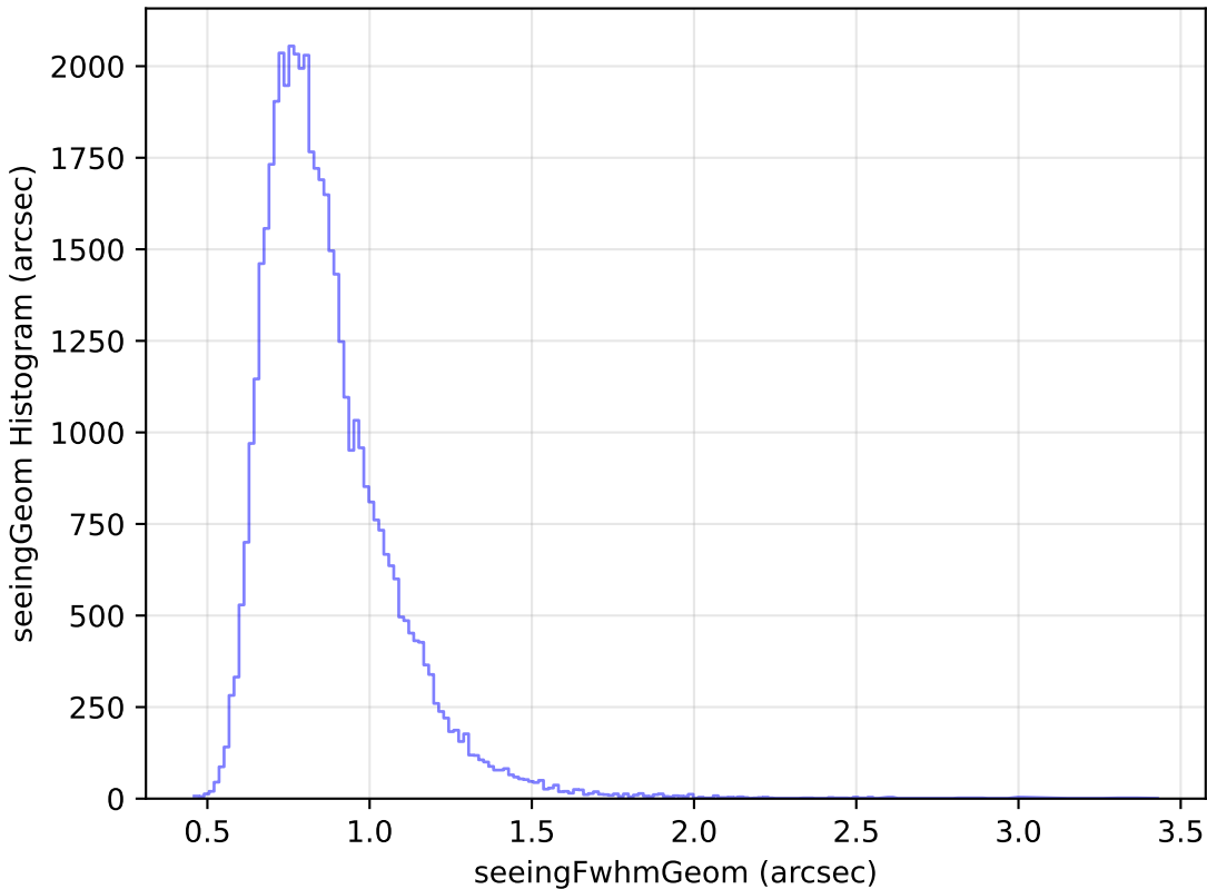
too_100_1v3.4_10yrs Yr 1 y band: seeingGeom Histogram
