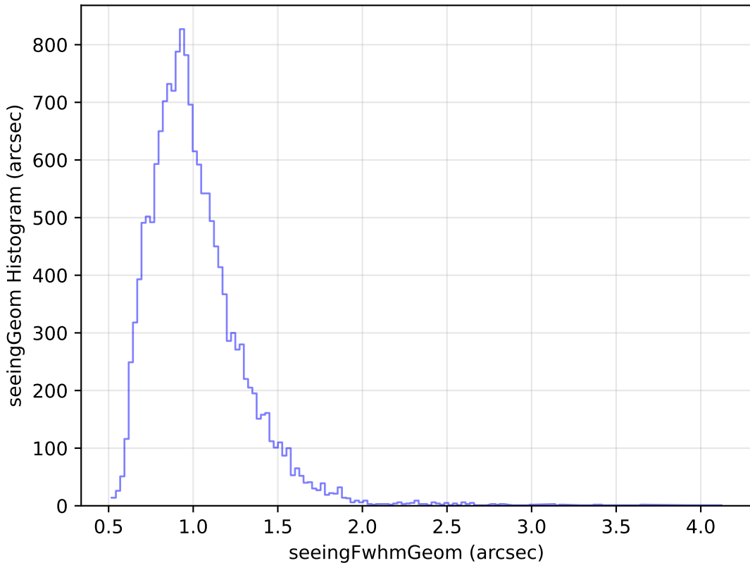
too_100_1v3.4_10yrs Yr 1 u band: seeingGeom Histogram
