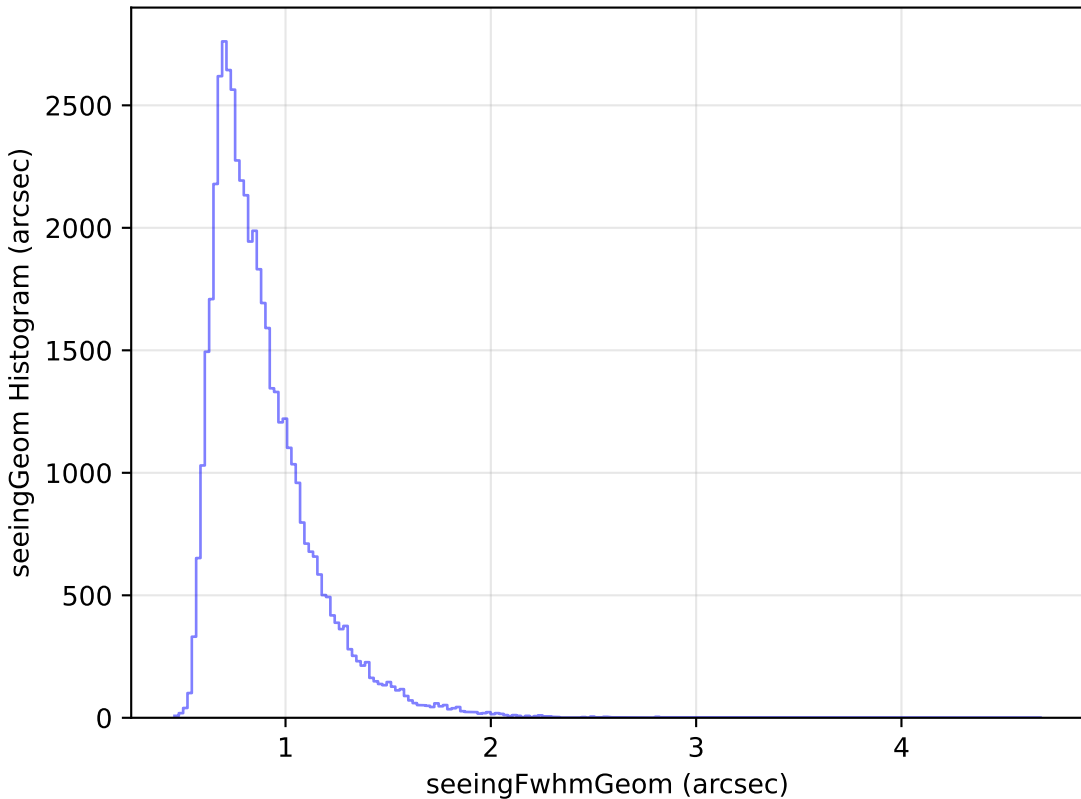
too_100_1v3.4_10yrs Yr 1 r band: seeingGeom Histogram
