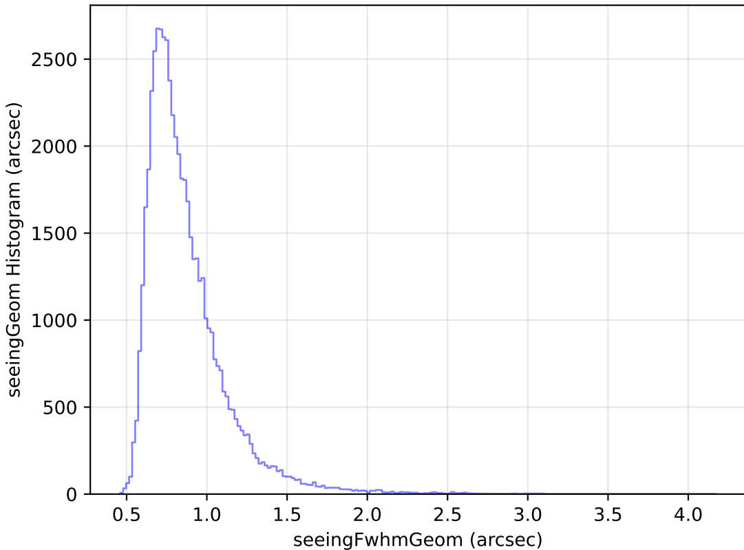
too_100_1v3.4_10yrs Yr 1 i band: seeingGeom Histogram
