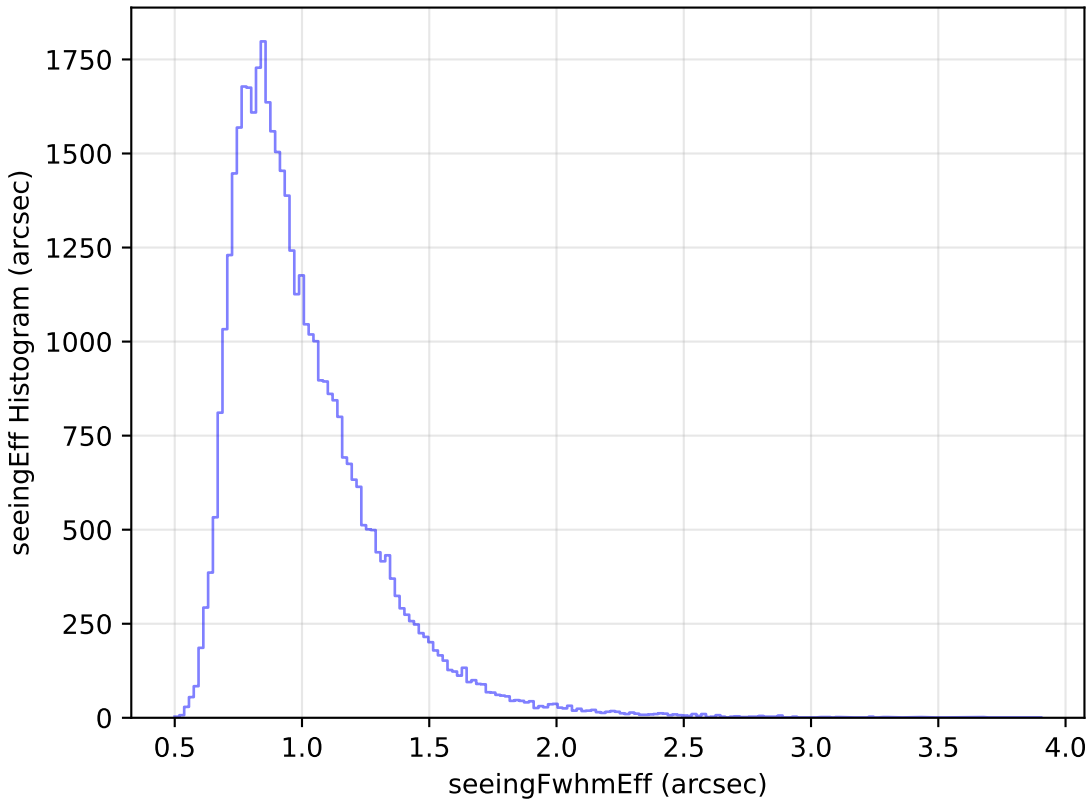
too_100_1v3.4_10yrs Yr 1 z band: seeingEff Histogram
