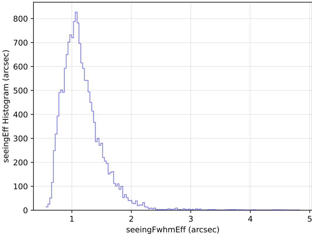
too_100_1v3.4_10yrs Yr 1 u band: seeingEff Histogram
