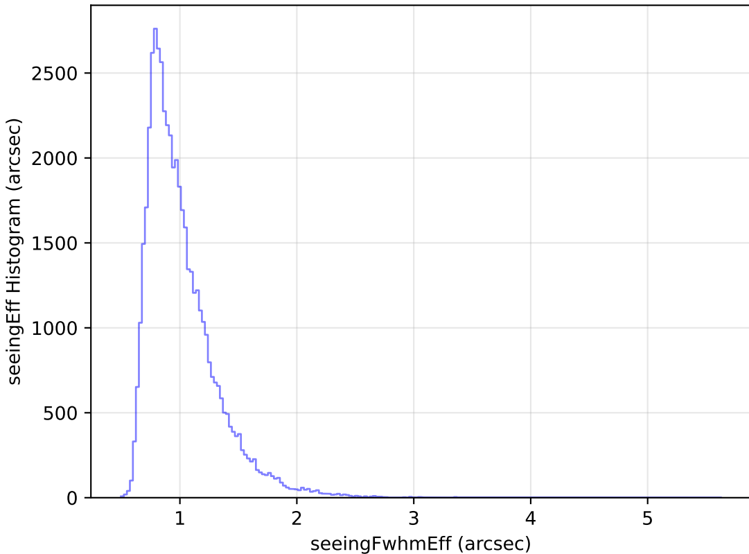
too_100_1v3.4_10yrs Yr 1 r band: seeingEff Histogram
