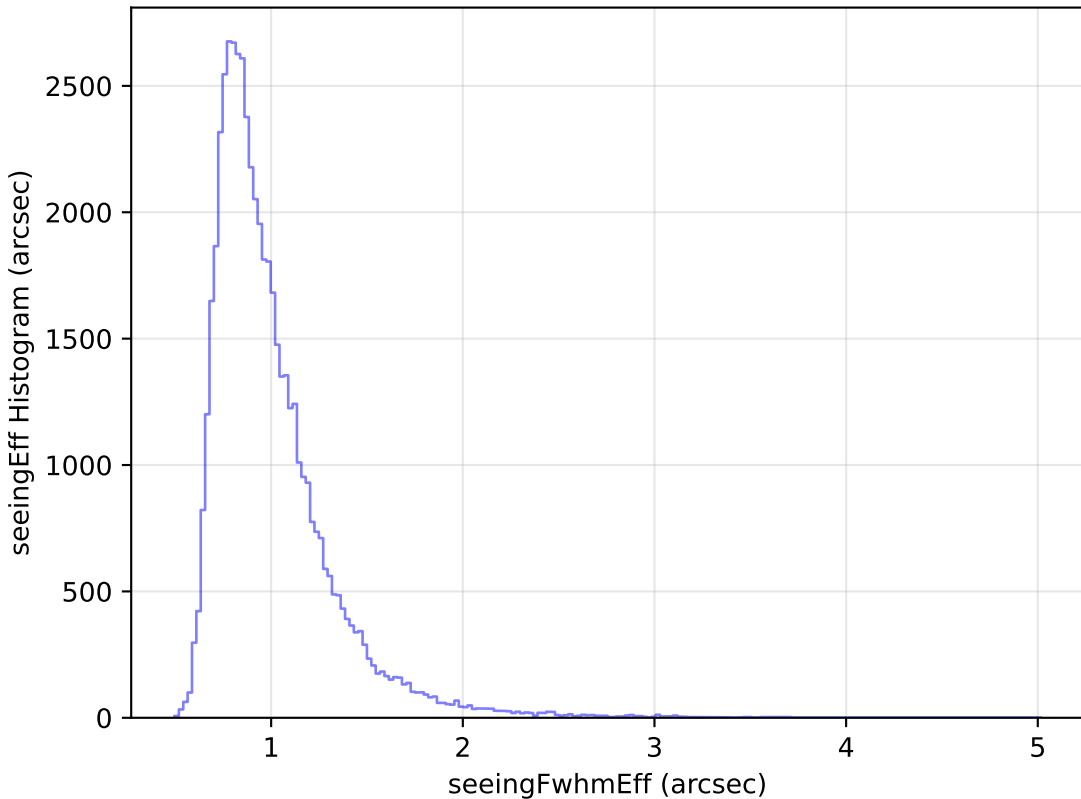
too_100_1v3.4_10yrs Yr 1 i band: seeingEff Histogram
