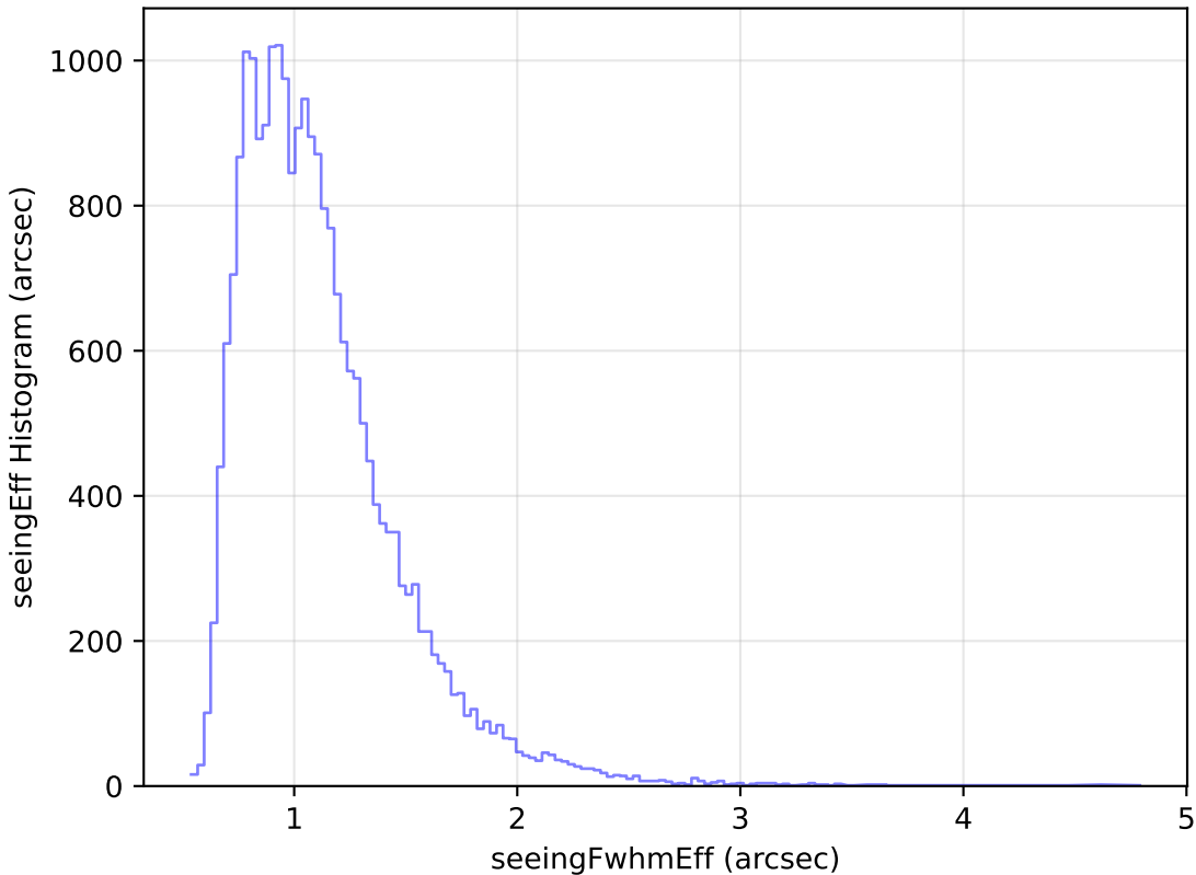
too_100_1v3.4_10yrs Yr 1 g band: seeingEff Histogram
