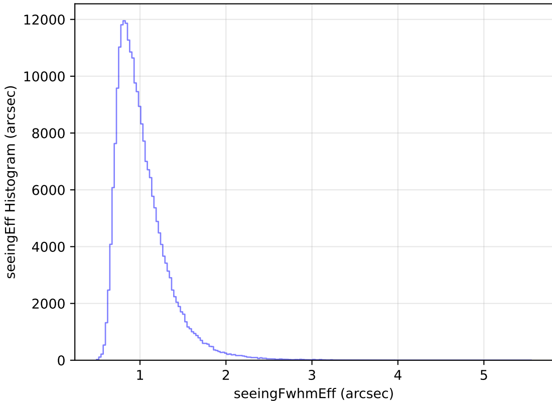
too_100_1v3.4_10yrs Yr 1 all bands: seeingEff Histogram
