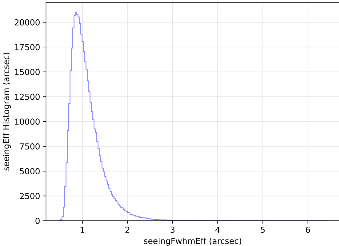
too_100_1v3.4_10yrs WFD z band: seeingEff Histogram
