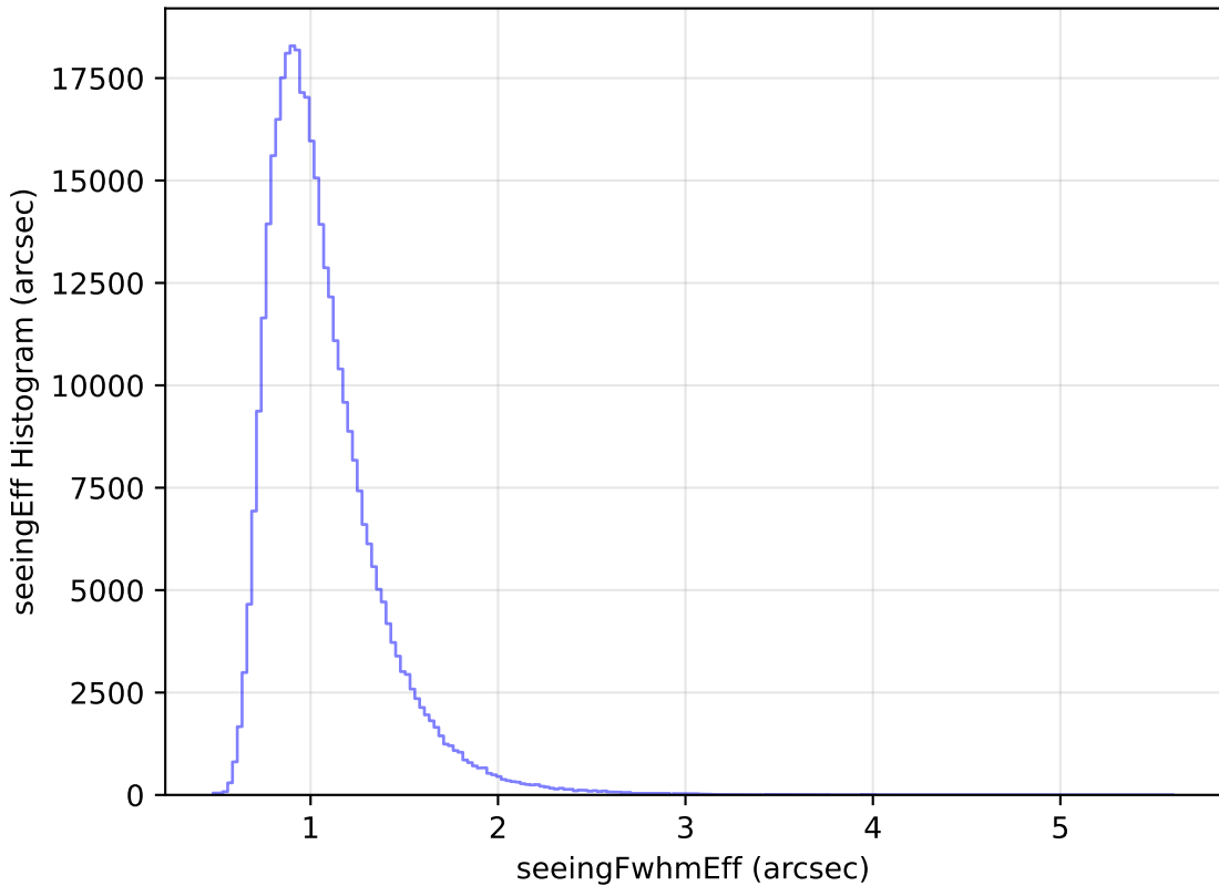
too_100_1v3.4_10yrs WFD y band: seeingEff Histogram
