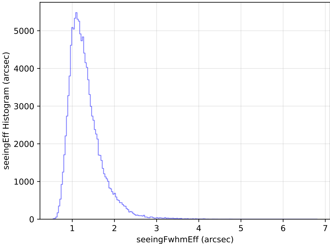
too_100_1v3.4_10yrs WFD u band: seeingEff Histogram
