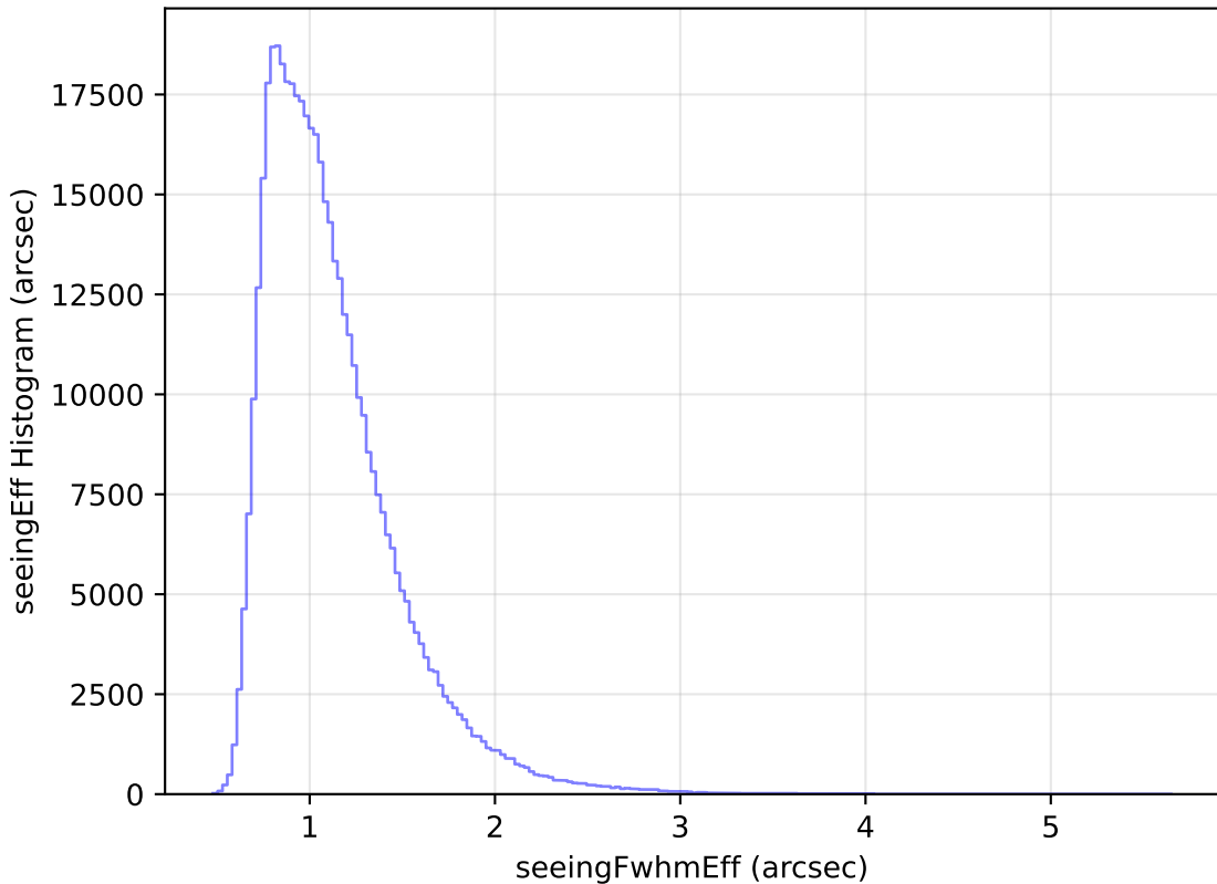
too_100_1v3.4_10yrs WFD r band: seeingEff Histogram
