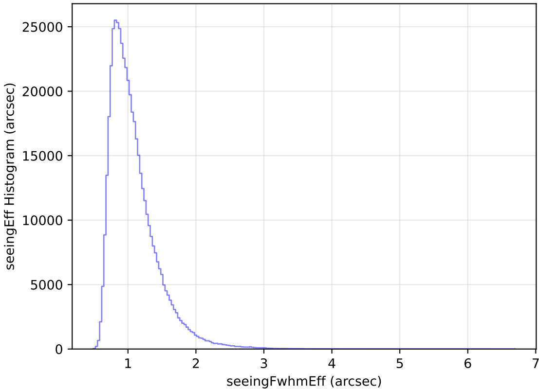
too_100_1v3.4_10yrs WFD i band: seeingEff Histogram
