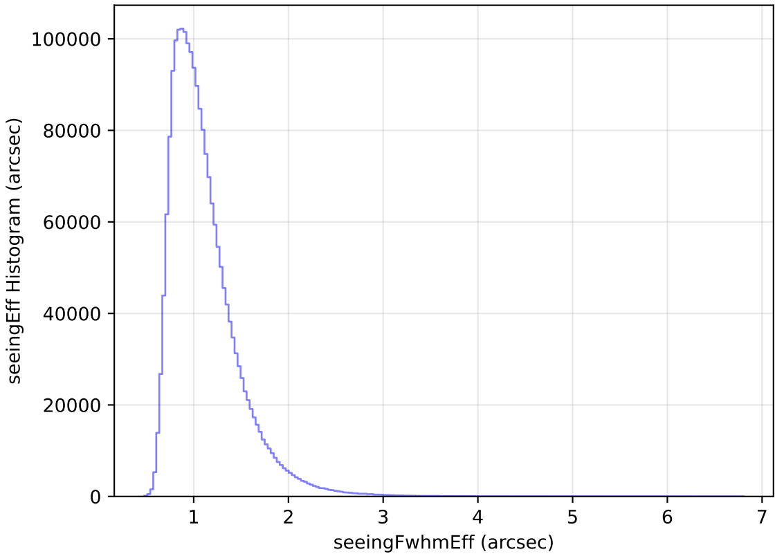
too_100_1v3.4_10yrs WFD all bands: seeingEff Histogram
