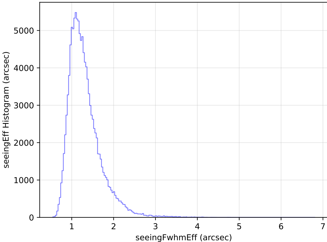
too_100_1v3.4_10yrs All sky u band: seeingEff Histogram
