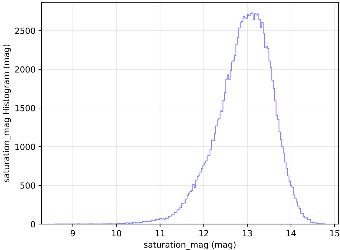
too_100_1v3.4_10yrs WFD u band: saturation_mag Histogram
