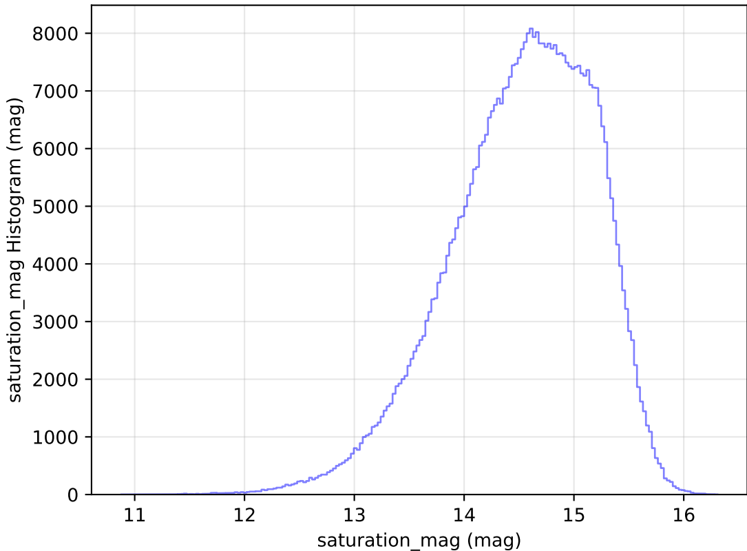
too_100_1v3.4_10yrs WFD r band: saturation_mag Histogram
