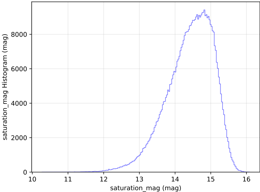
too_100_1v3.4_10yrs WFD i band: saturation_mag Histogram
