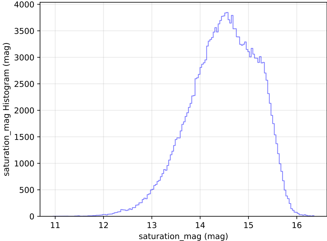
too_100_1v3.4_10yrs WFD g band: saturation_mag Histogram
