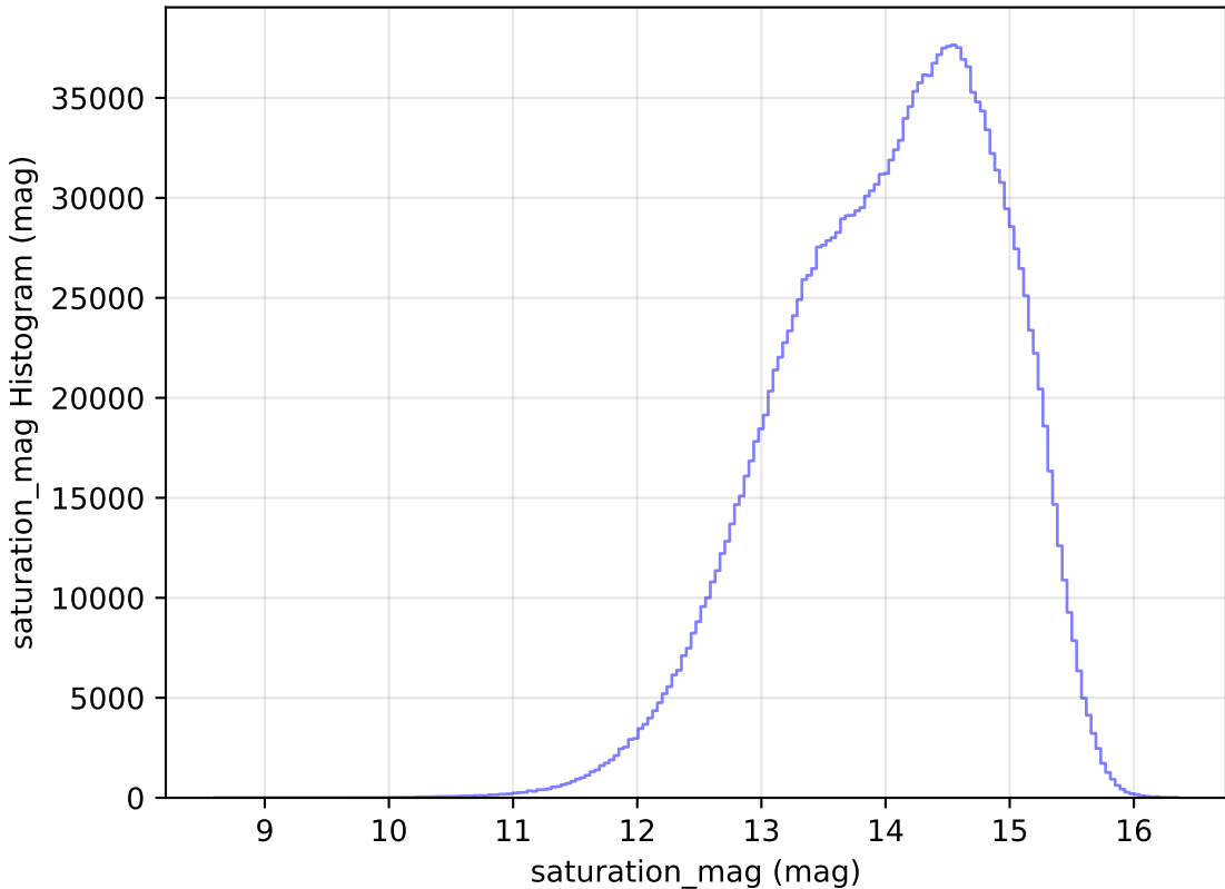
too_100_1v3.4_10yrs WFD all bands: saturation_mag Histogram
