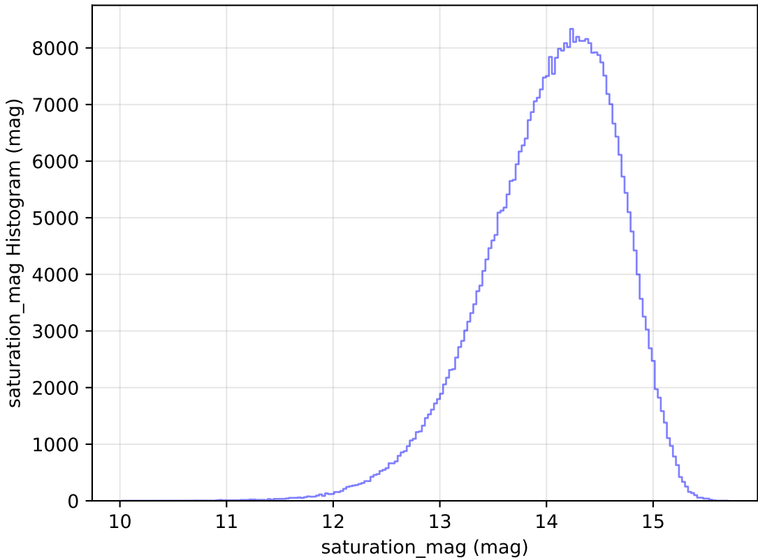
too_100_1v3.4_10yrs All sky z band: saturation_mag Histogram
