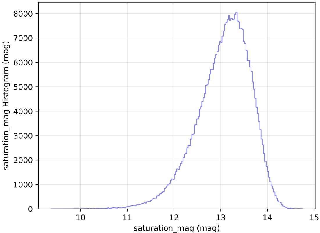
too_100_1v3.4_10yrs All sky y band: saturation_mag Histogram
