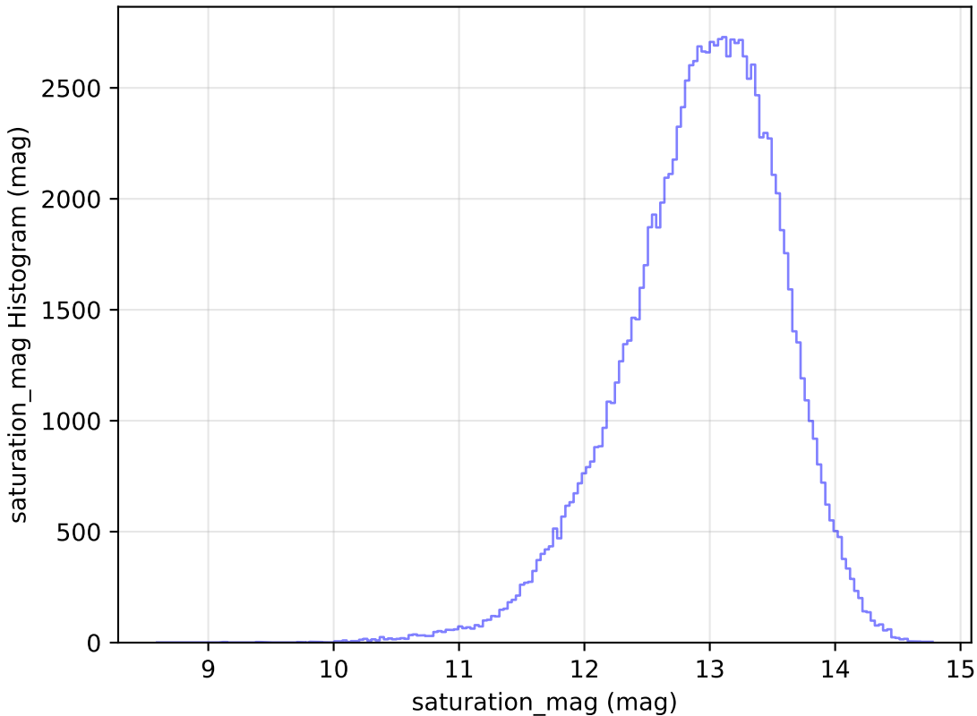
too_100_1v3.4_10yrs All sky u band: saturation_mag Histogram
