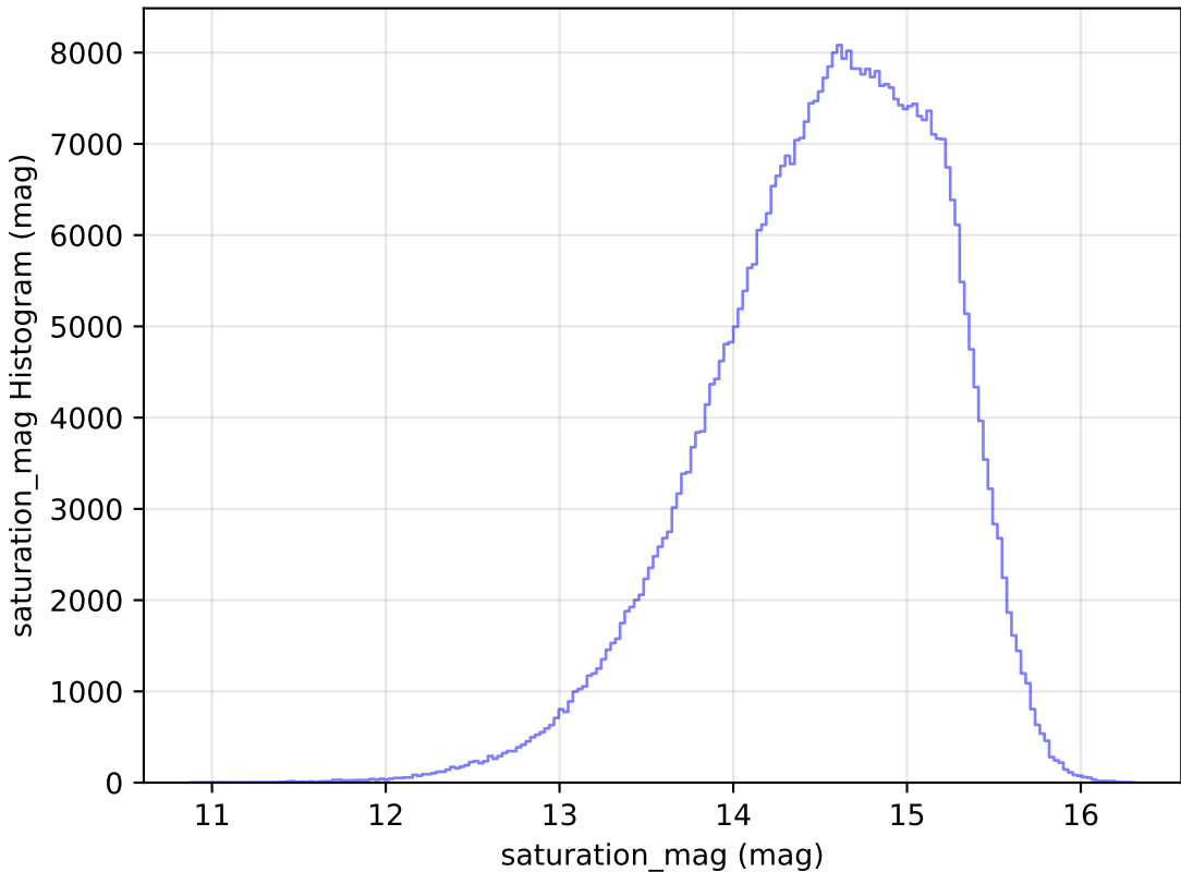
too_100_1v3.4_10yrs All sky r band: saturation_mag Histogram
