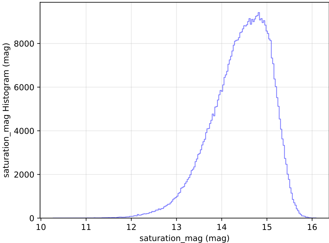
too_100_1v3.4_10yrs All sky i band: saturation_mag Histogram
